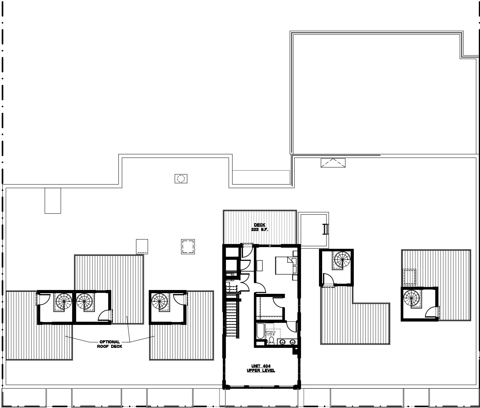
FIFTH FLOOR PLAN / ROOF PLAN
